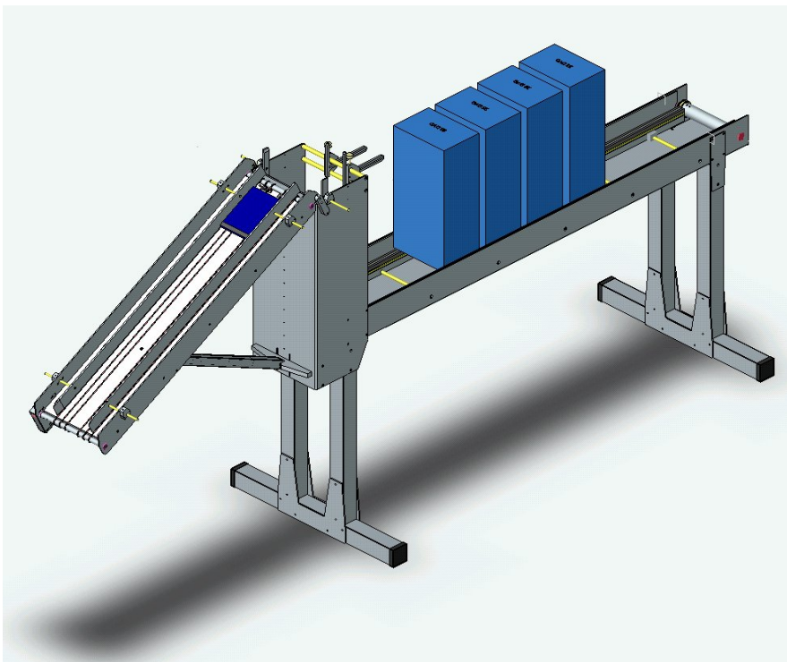
Universal Servo Product Stacker Showing Products Stacked on Out- Feed Conveyor and One Product on In-Feed Conveyor
